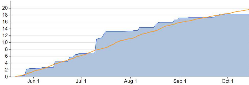
Accumulated Precipitation
