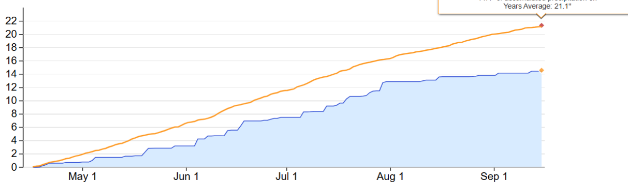
Accumulated Precipitation
