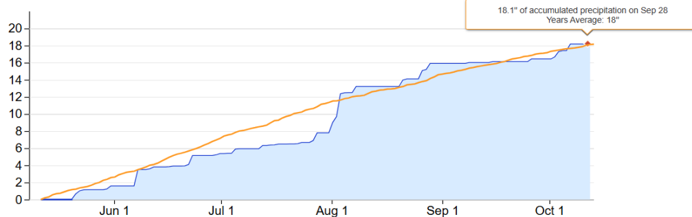
Accumulated Precipitation
