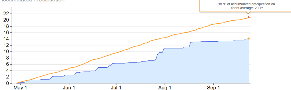
Accumulated Precipitation
